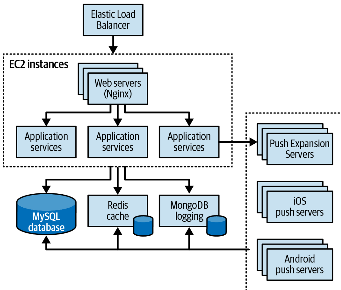
Figure 22-5. Example architecture diagram for risk storming session
