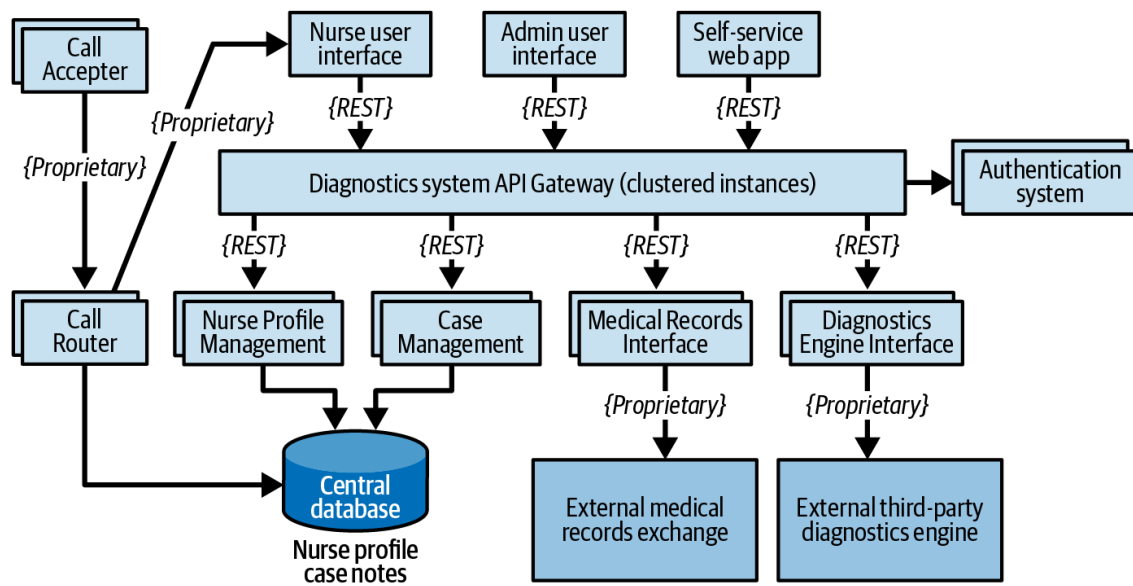
Figure 22-8. High-level architecture for a nursing-hotline diagnostics system
