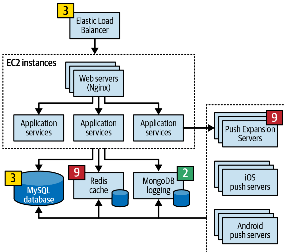
Figure 22-7. Consensus of risk areas
