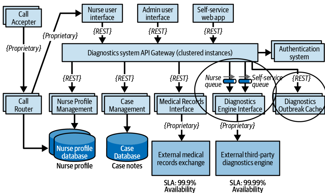
Figure 22-11. Architecture modifications to address elasticity risk
