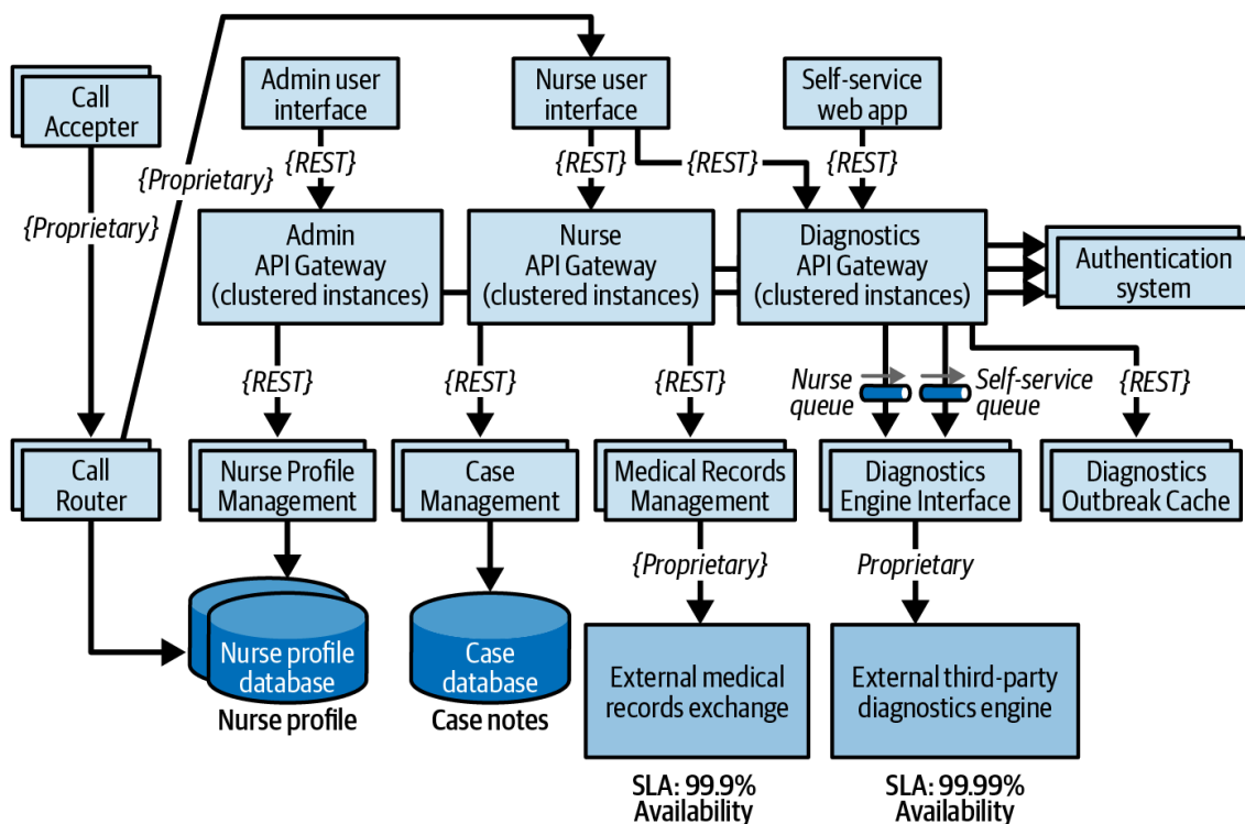
Figure 22-12. Architecture modifications to address security risk
