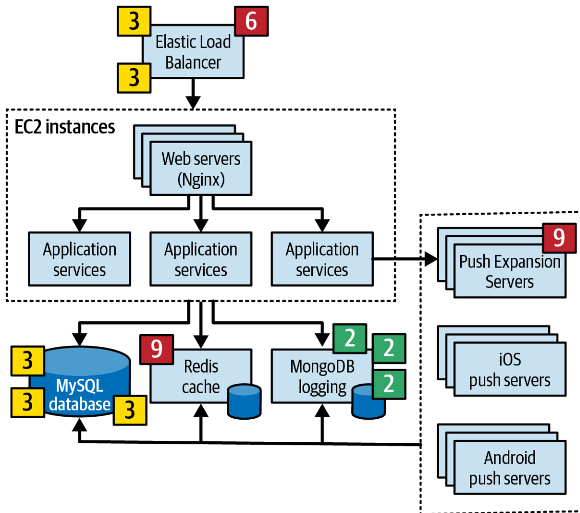
Figure 22-6. Initial identification of risk areas
